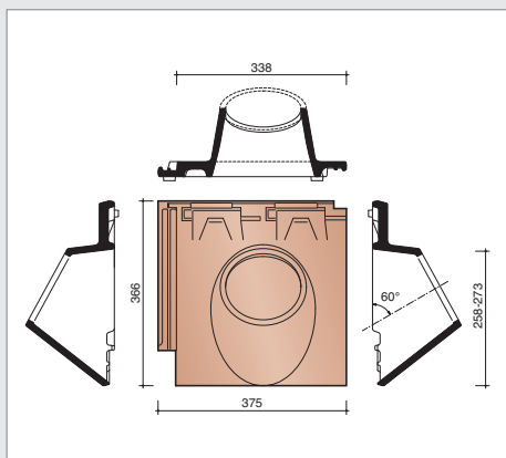
MVBD8770 Kokerpan Ø 150 mm
